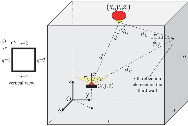
Fig. 2. Single-LED-based VLC channel model.
