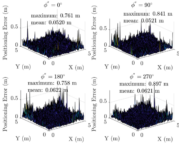
Fig. 19. Positioning error distribution of the proposed LS-IGWO positioning algorithm when \phi' = 15^\circ and SNR = 20 dB for different \phi'' values.
