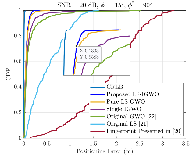
Fig. 20. CDF of the positioning error for the six investigated positioning algorithms (considering the LED orientation).
